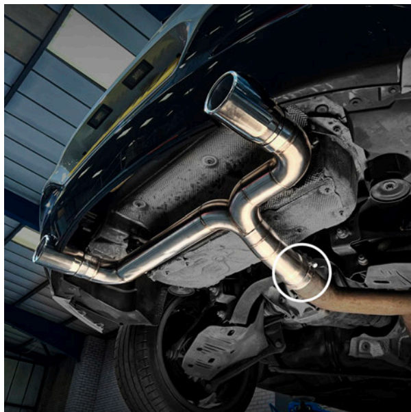
8. The Backbox sleeves over the OEM Exhaust.
